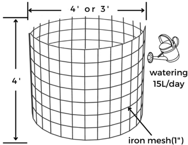
Compost Pile
